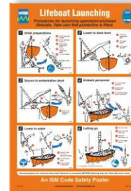
Lifeboat Launching
